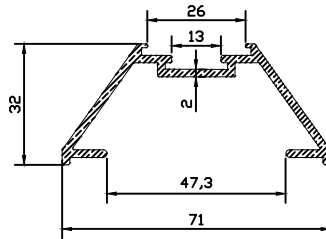
10296 0.753 kg/m
