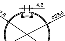
9561 0.322 kg/m
