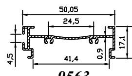
9563 0.304 kg/m
